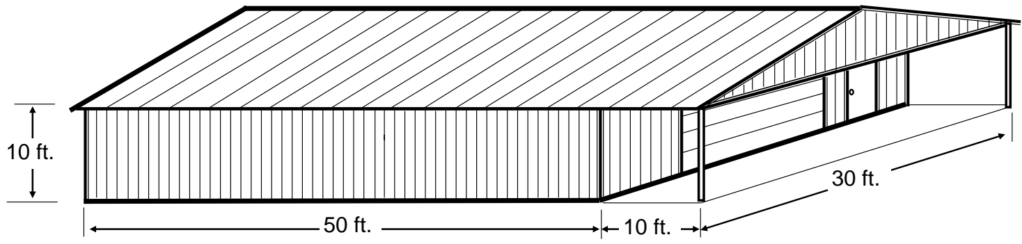
Front View
